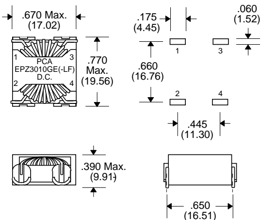
Package
