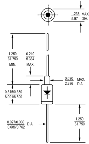
All dimensions in \frac{\text{INCH}}{\text{m.m.}} DO-13 (DO-202AA)
