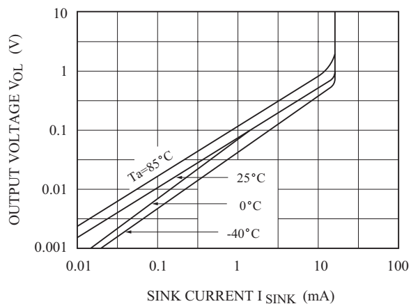
V_{OL} - I_{SINK}
