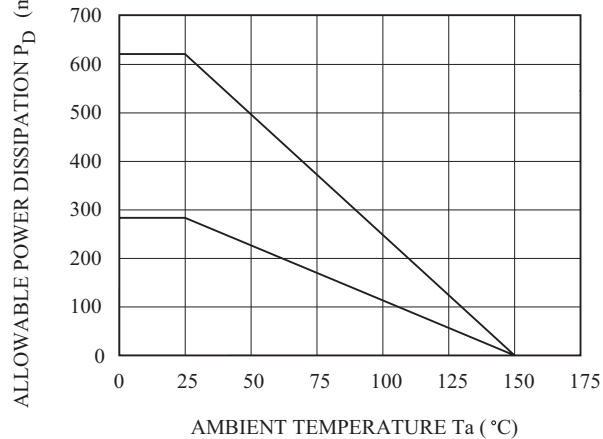
P_D - T_a
