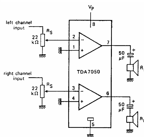
Application diagram (stereo)
