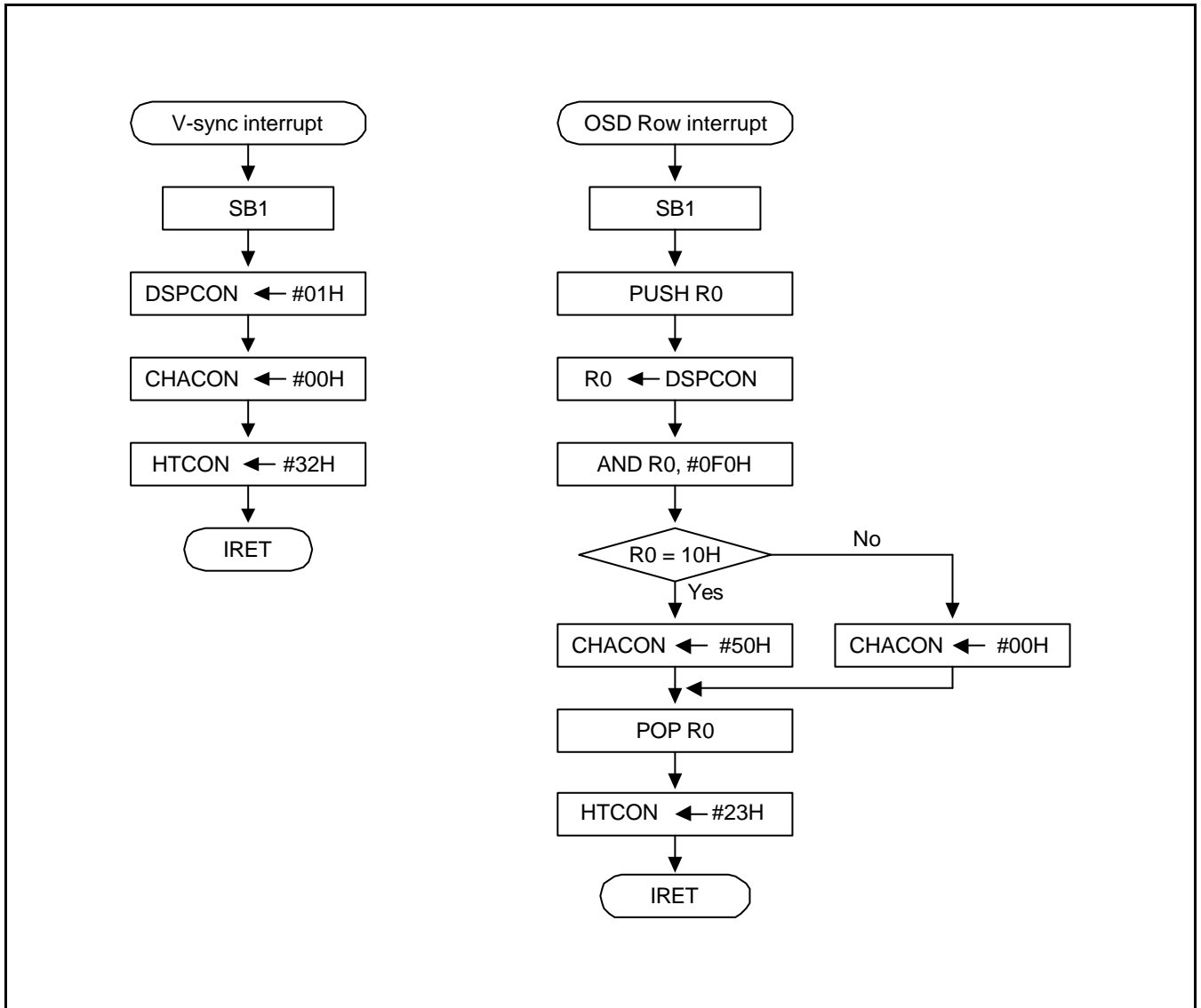
Figure 13-37. Decision Flowchart for Row Interrupt Function Programming Tip
