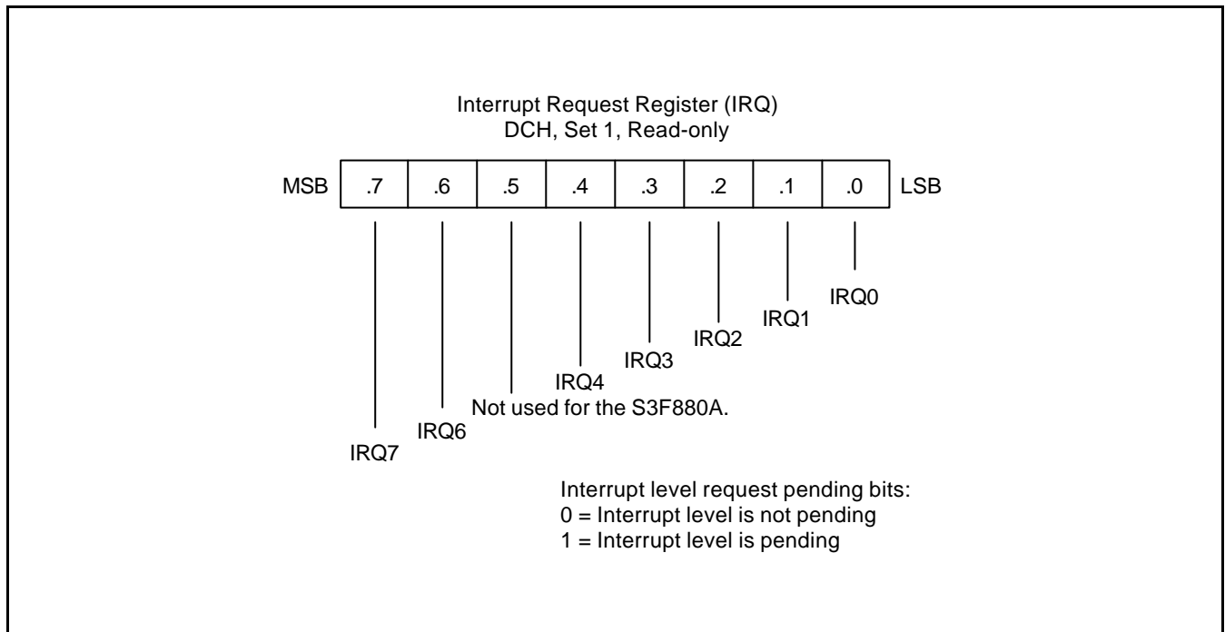
Figure 5-8. Interrupt Request Register (IRQ)
