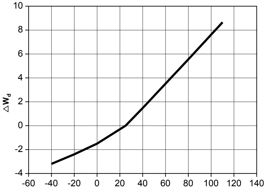
Fig 8. Dominant wavelength shift vs. Junction Temperature, I_F = 50\text{mA}
