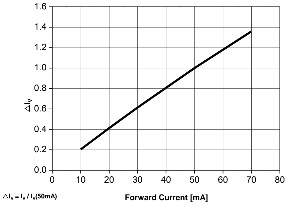
Fig 4. Forward Current vs. Relative Luminous Intensity, T_j = 25^\circ\text{C}
