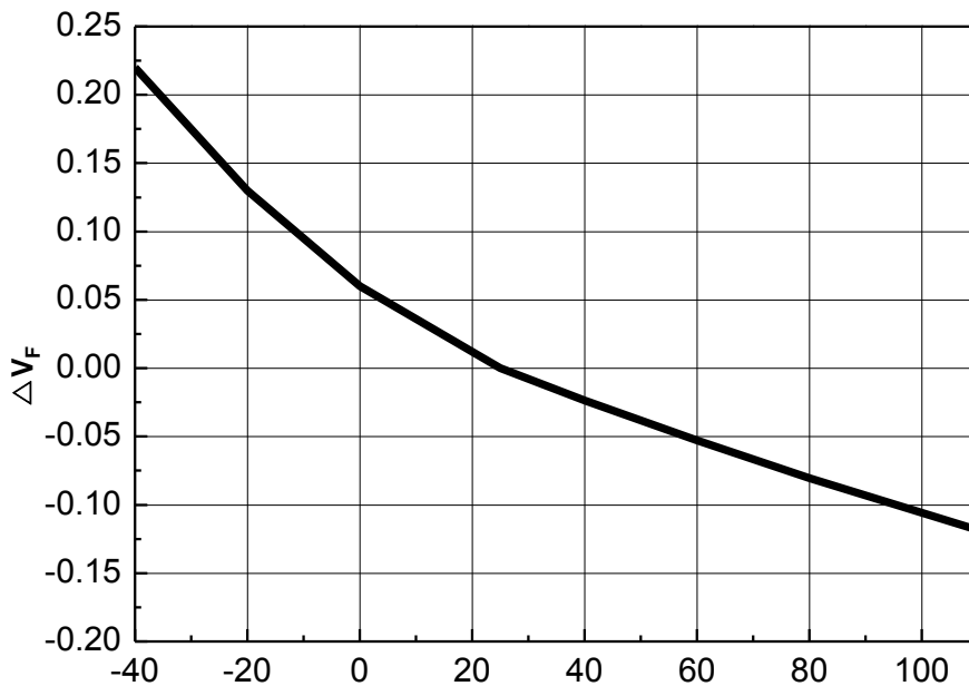
Fig 7. Junction Temperature vs. Forward Voltage shift, I_F = 50\text{mA}
