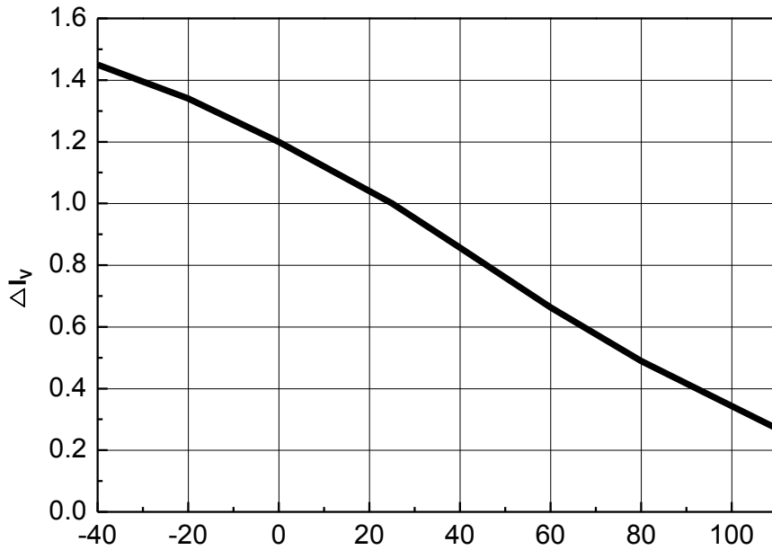
Fig 6. Relative Light Output vs. Junction Temperature, I_F = 50\text{mA}
