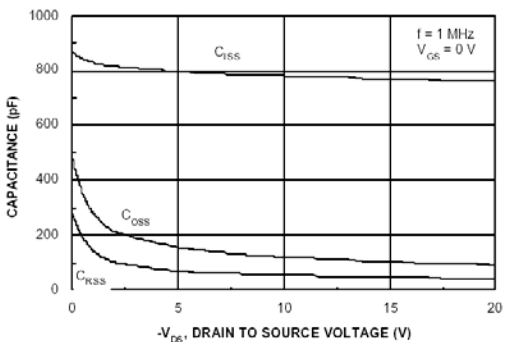
Figure 8. Capacitance Characteristic
