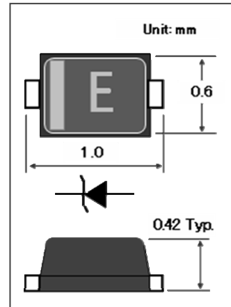
Fig -1 Package SOD923
