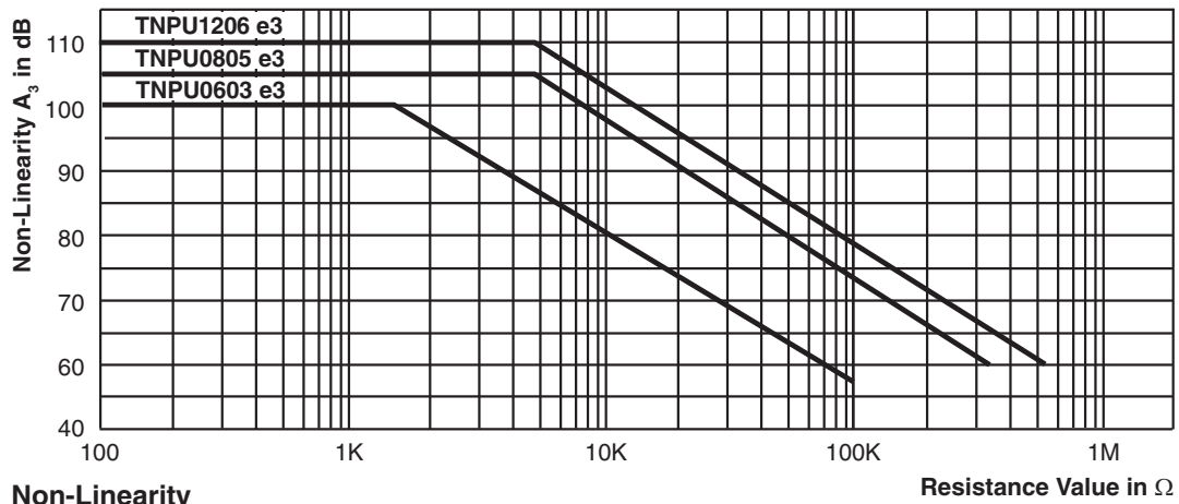
Non-Linearity
