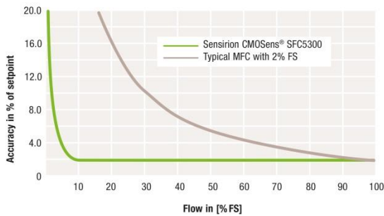
Figure 4: Accuracy comparison of the CMOSens® SFC5300 / SFM5300 device compared to a typical thermal mass flow controller / meter.
