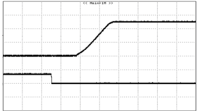
Figure 14: Turn on Using Remote On/Off with external capacitors ( C_o= 3000 \mu F ), 5.0V/5A out (resistive load)(10mS/div) Top trace: Vout,2V/div; Bottom trace: ON/OFF,5V/div
