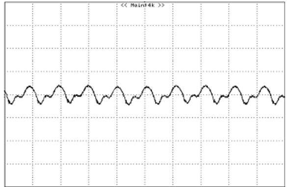
Figure 8: Output ripple & noise at 12Vin, 2.5V/5A out 50mV/div, pk-pk : 17.50mV, rms : 4.67mV(20mV/div,2uS/div)
