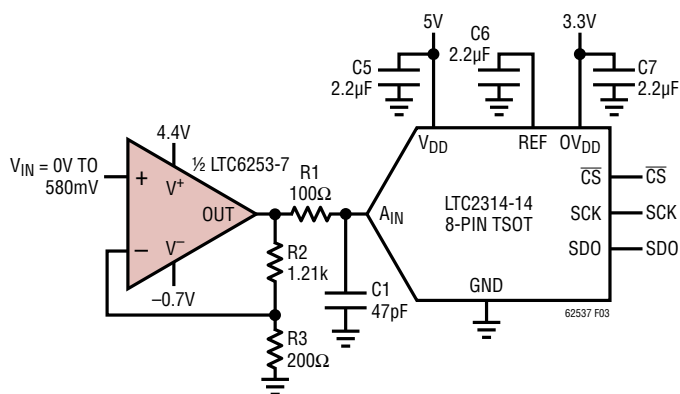
Figure 3. ADC Driver with Gain
