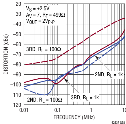
Distortion vs Frequency, 5V Supply
