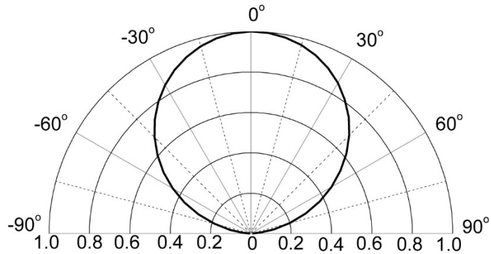
Figure5. Relative Luminosity VS. Radiation Angle
