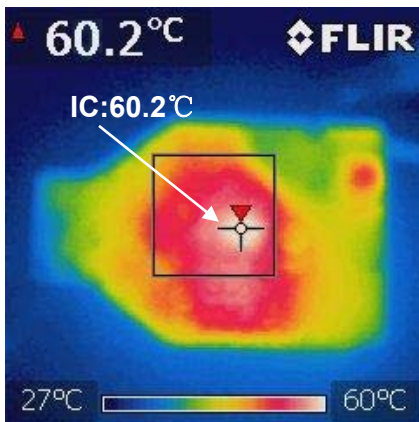
Without dimmer @ V IN =108V AC
