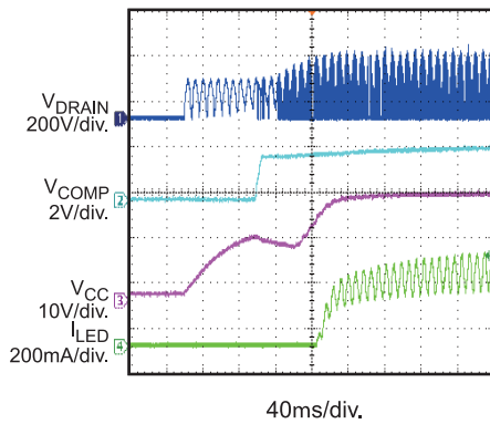
V_{IN} Start-Up
