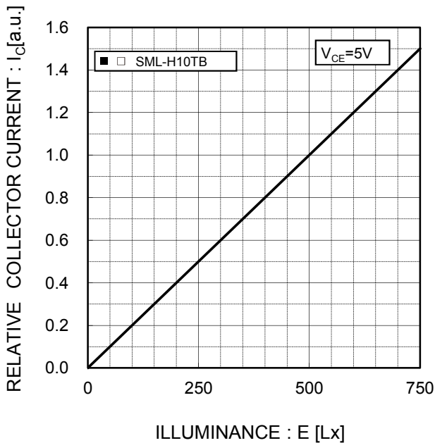
Fig.3 Relative Collector Current - Illuminance
