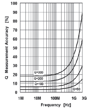
Q accuracy @ 7-mm port (typical)
