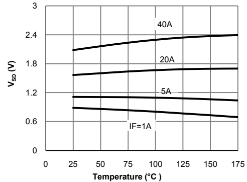
Fig 20: Diode Forward Voltage vs. Junction Temperature
